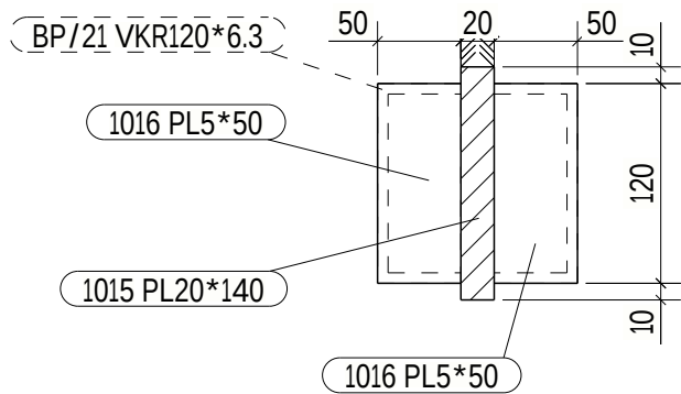
A - A 1:5
